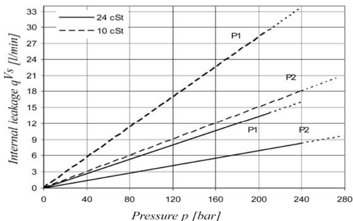
INTERNAL LEAKAGE (TYPICAL)
