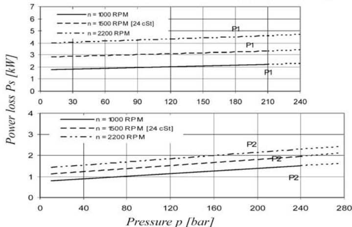
HYDROMECHANICAL POWER LOSS (TYPICAL)
