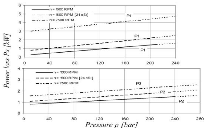
HYDROMECHANICAL POWER LOSS (TYPICAL)
