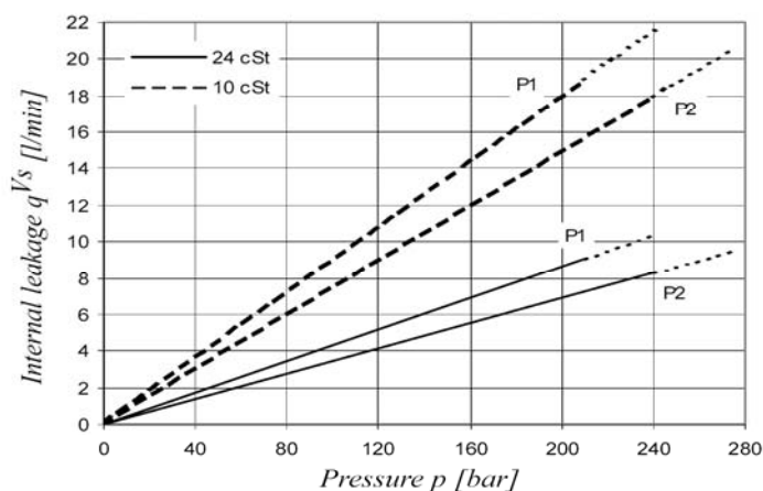
INTERNAL LEAKAGE (TYPICAL)
