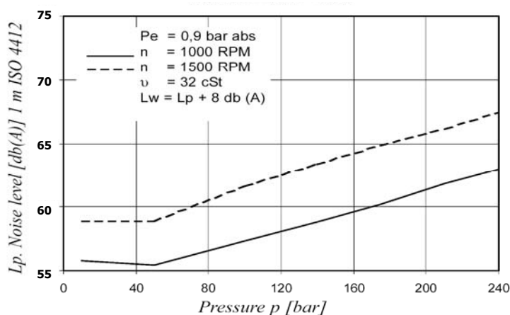
NOISE LEVEL (TYPICAL)
