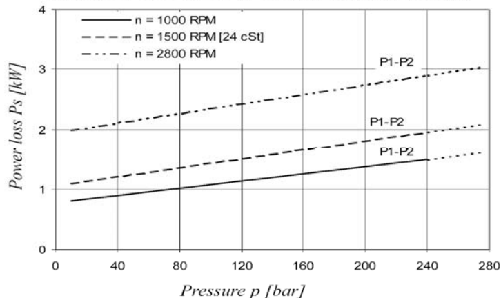
HYDROMECHANICAL POWER LOSS (TYPICAL)
