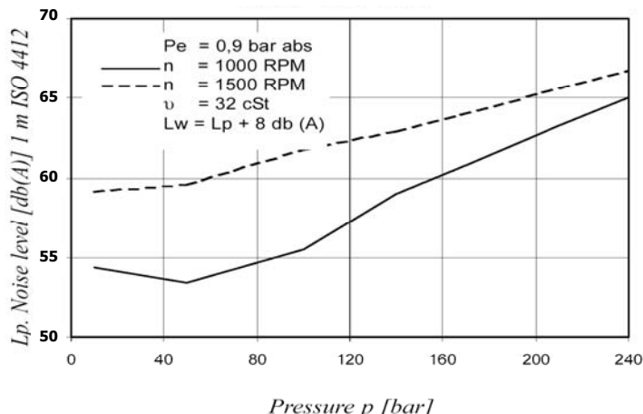
NOISE LEVEL (TYPICAL)
