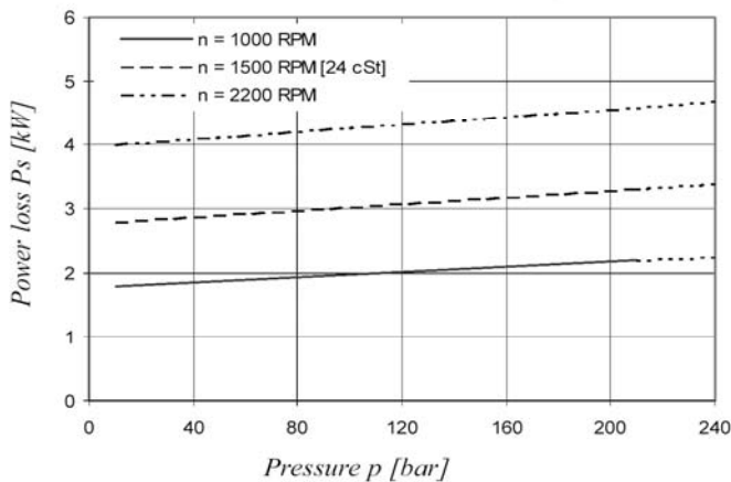
HYDROMECHANICAL POWER LOSS (TYPICAL)
